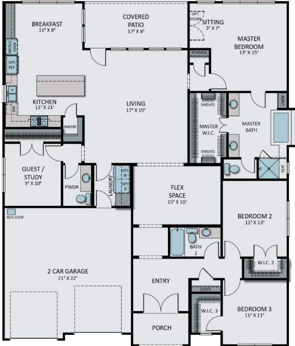
Elevation A Floorplan
