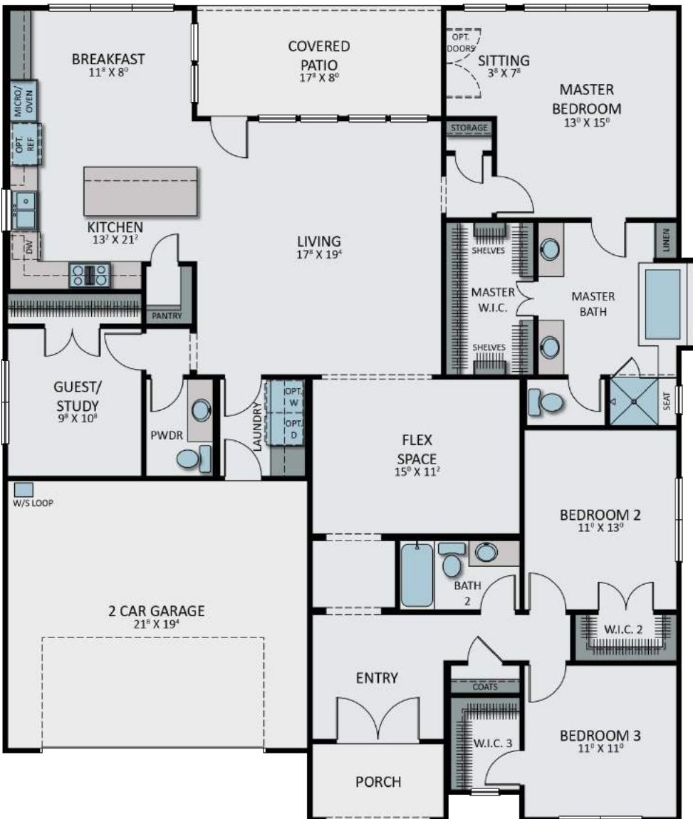
Elevation B Floorplan
