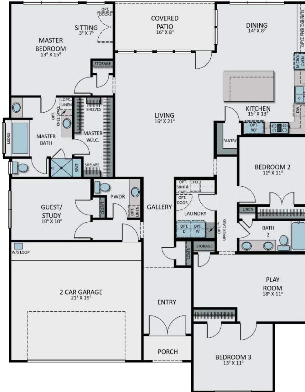
Elevation B Floorplan
