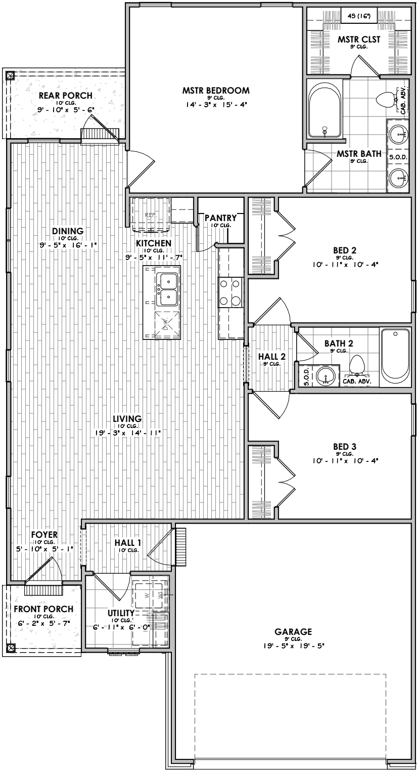
FLOOR PLAN OVERALL DIMENSIONS 34' - 1" WIDTH X 63' - 2" DEPTH
