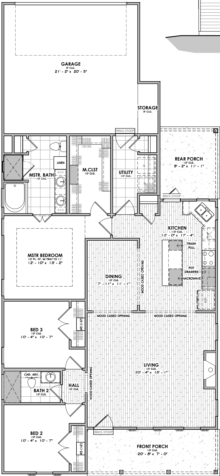
FLOOR PLAN
