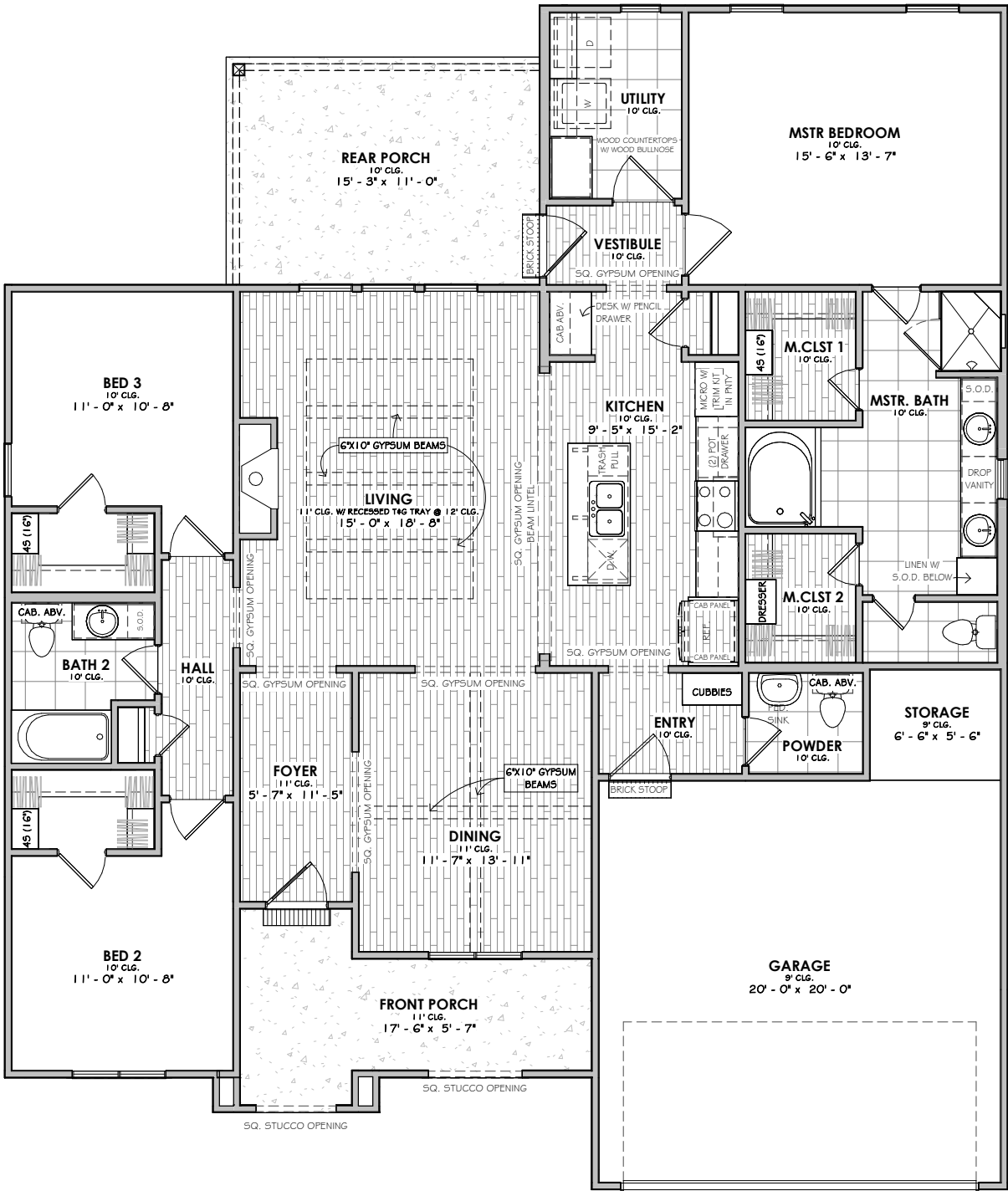
FLOOR PLAN
