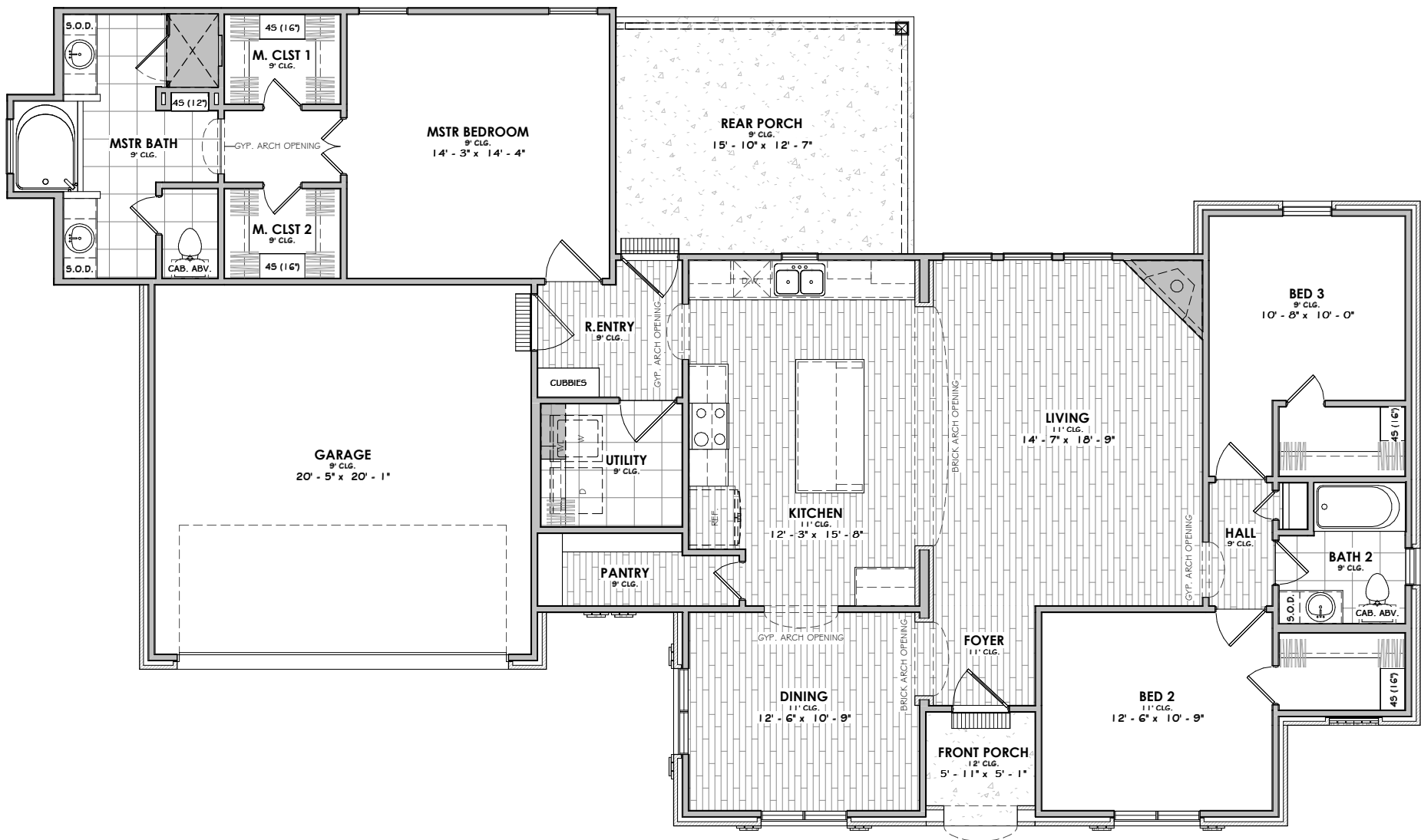
FLOOR PLAN
