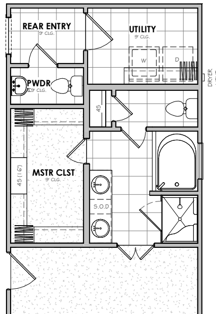
ENLARGED MASTER CLOSET W/ POWDER OPTION
