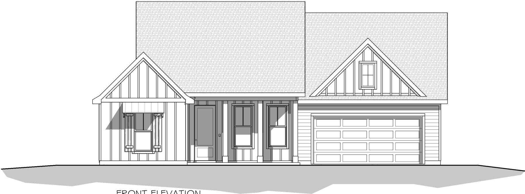
FRONT ELEVATION 9'-1" # 10'-1" PLATE HEIGHT - 9' # 10' CLG. 9:12 # 12:12 ROOF PITCH
