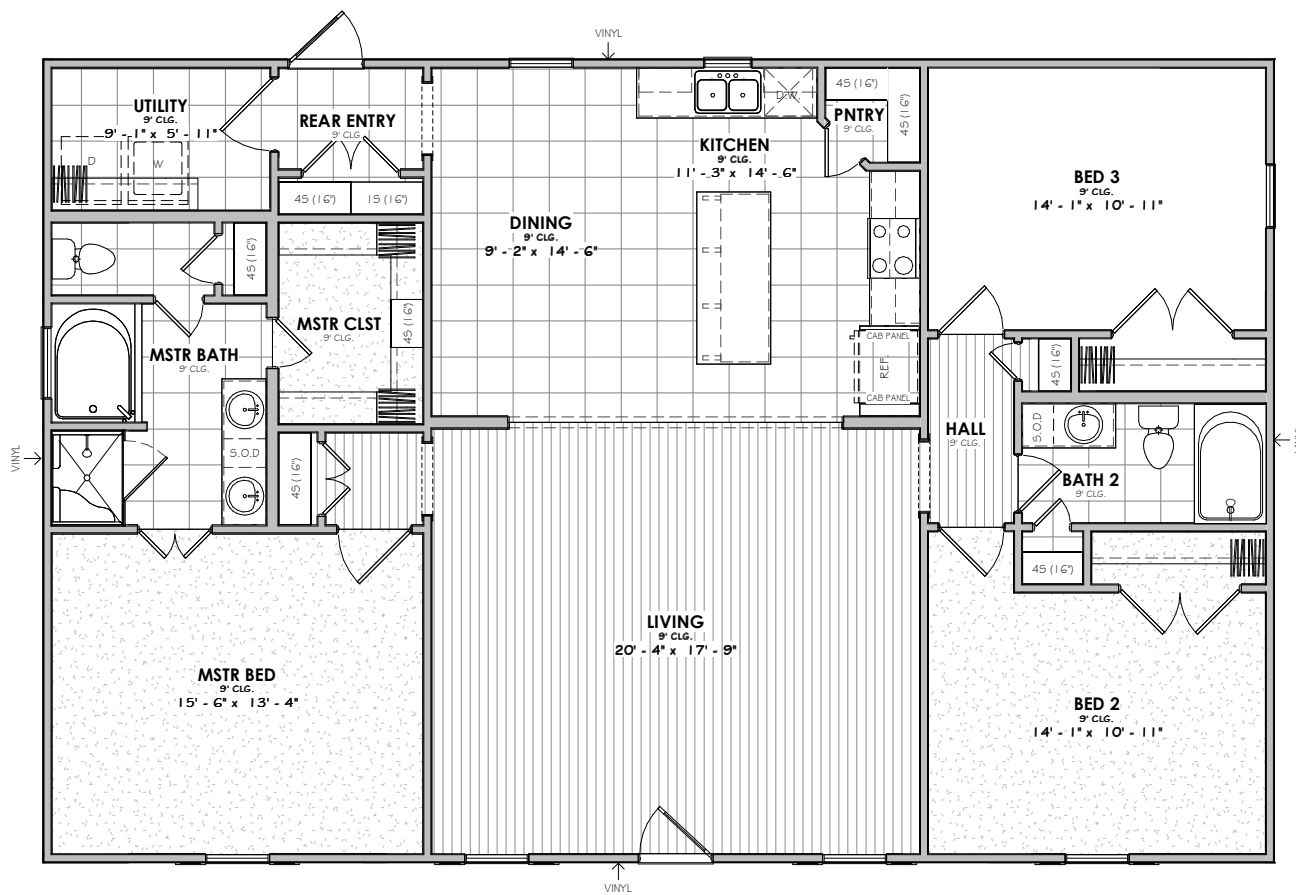
FLOOR PLAN
