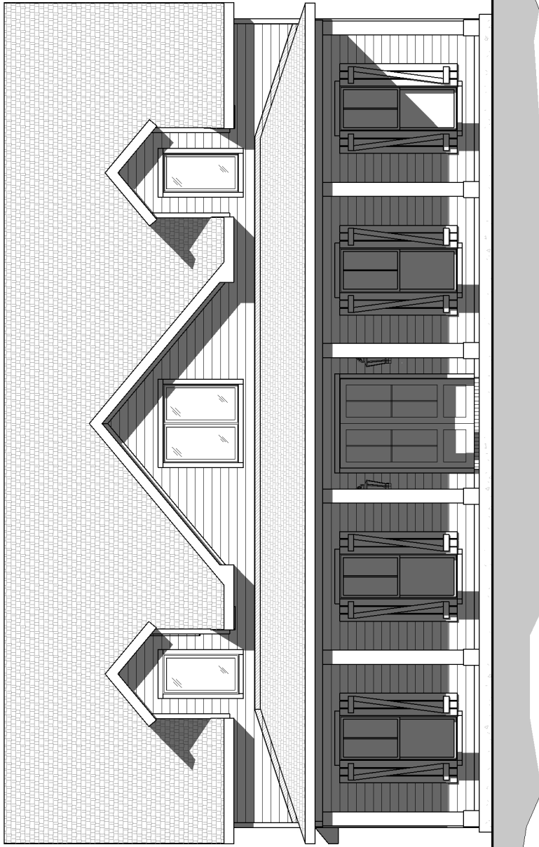
FRONT ELEVATION 10'-11" x 15'-11" PLATE HEIGHTS - 9' CLG., 1st FLOOR x 9' CLG., 2nd FLOOR 10:12 ROOF PITCH
