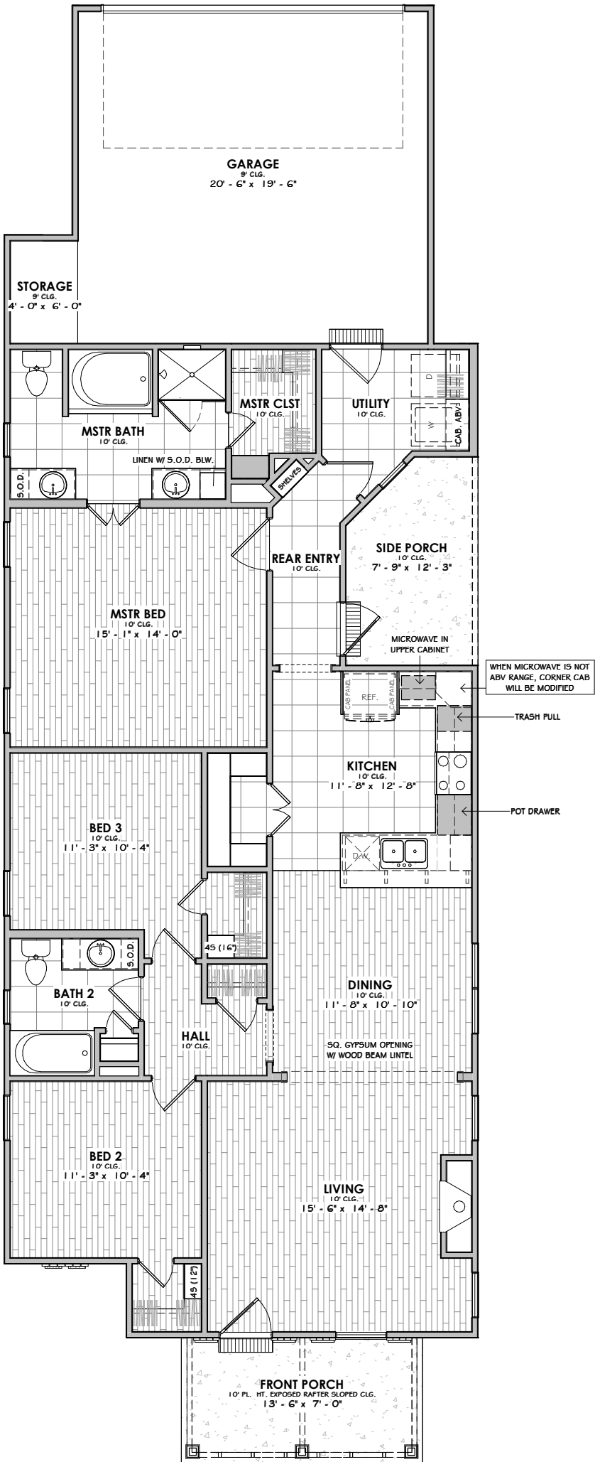
FLOOR PLAN
