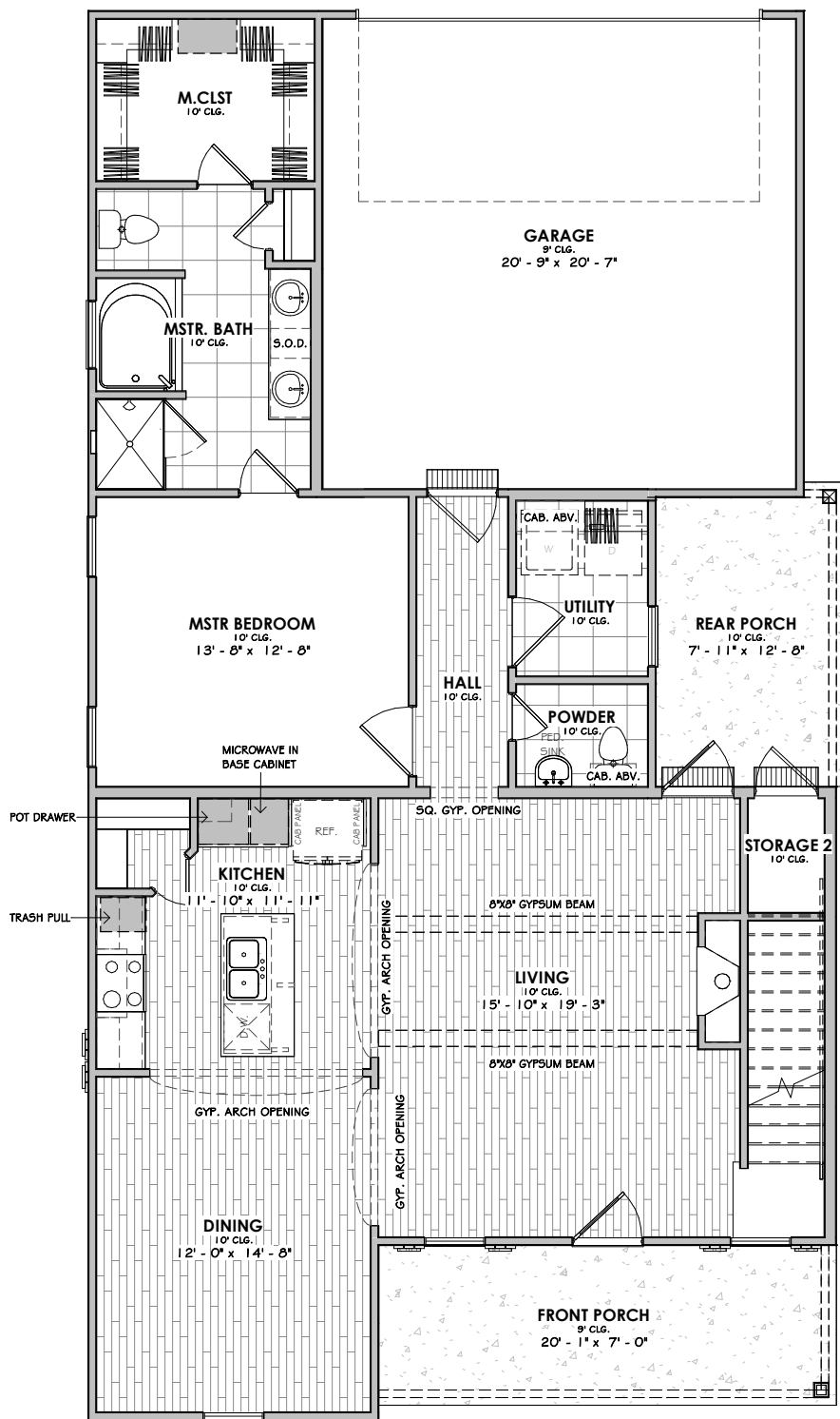
FLOOR PLAN
