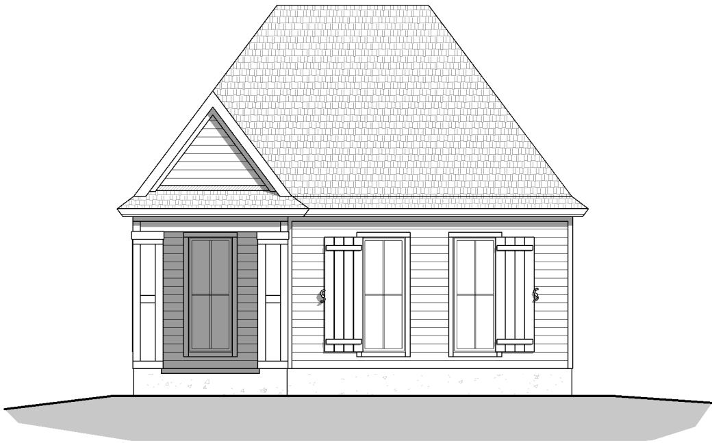
FRONT ELEVATION 10'-1" PLATE HEIGHT - 9', 10' CLG. 9:12; 16:12 ROOF PITCH
