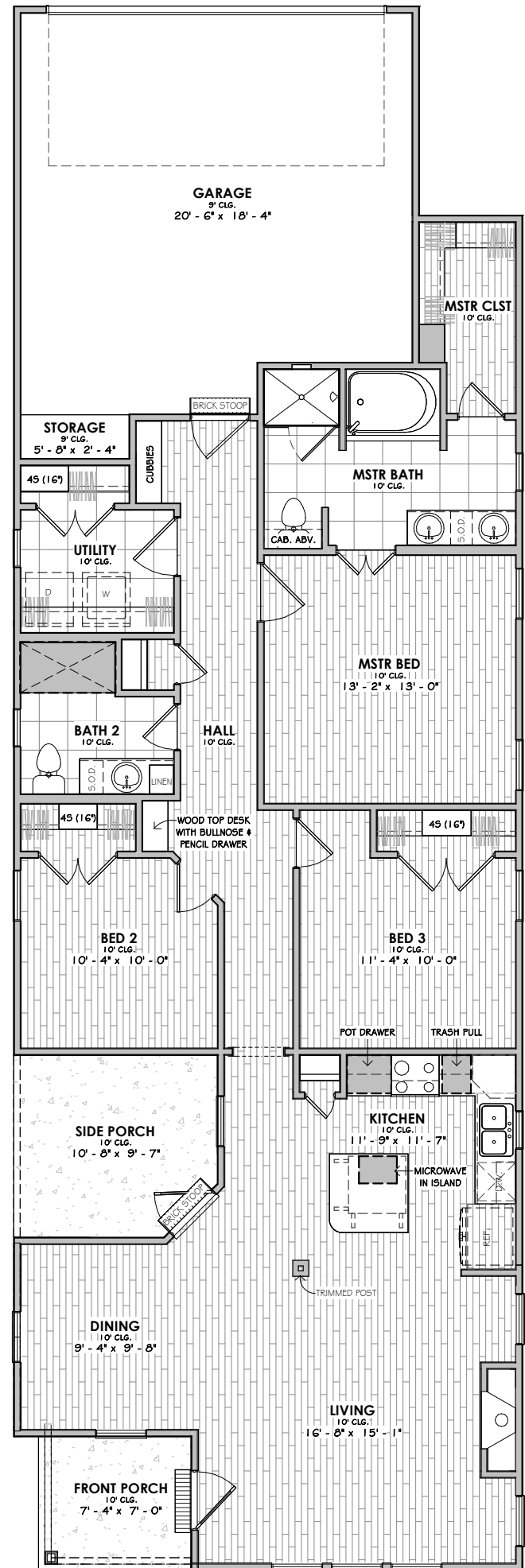
FLOOR PLAN
