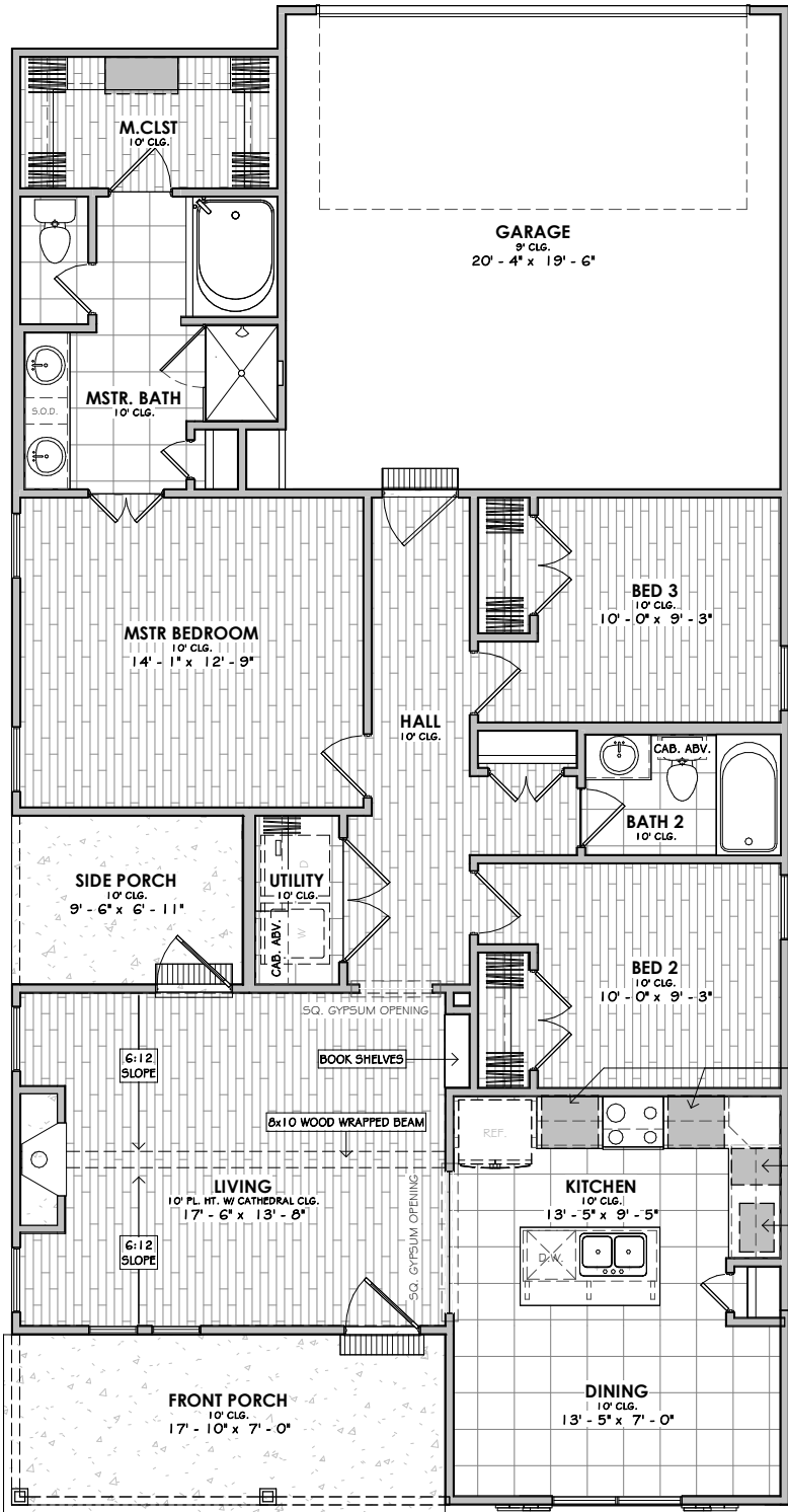
FLOOR PLAN OVERALL DIMENSIONS 32'-4" WIDTH X 62'-0" DEPTH
