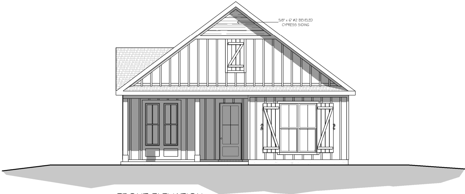
FRONT ELEVATION 10'-1" PLATE HEIGHT - 9' 4 10' CLG. 9:12 ROOF PITCH
