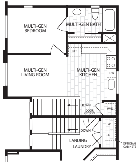
MULTI-GEN OPTION SECOND FLOOR
