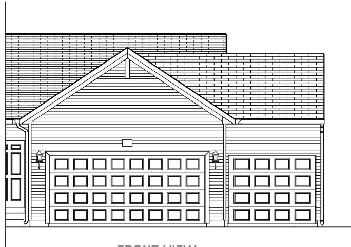
FRONT VIEW 10' X 20' 3 CAR GARAGE OPTION *20 x 24 GARAGE OPTION REQUIRED
