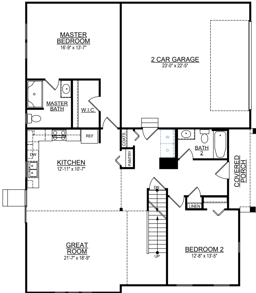
FIRST FLOOR
