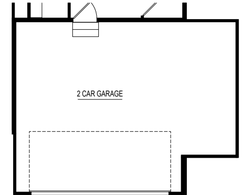
6' X 16' GARAGE BUMP OPTION
