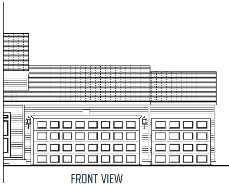
FRONT VIEW 20' X 24' GARAGE OPTION
