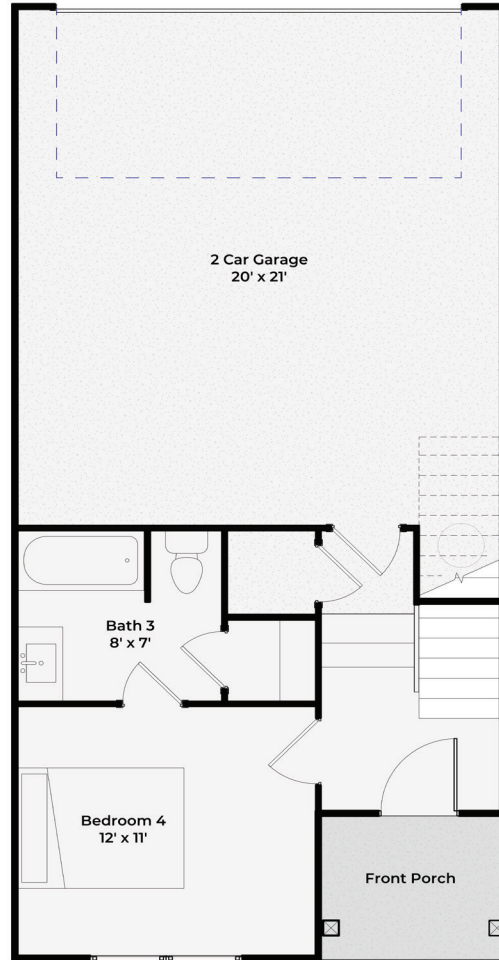
Optional Bedroom and Full Bath
