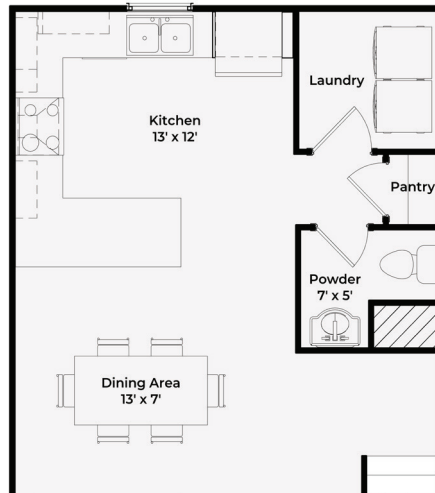
Optional Kitchen Layout B
