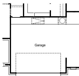
2 1/2 Car Garage
