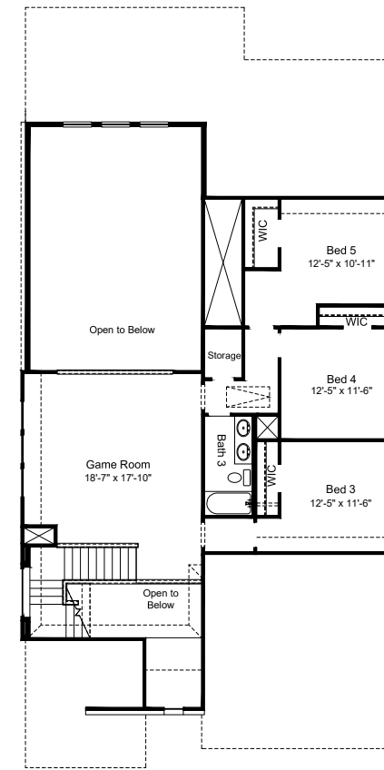
2nd Floor
