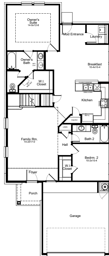
1st Floor
