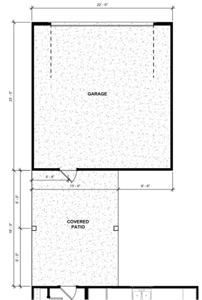
OPT. ATTACHED GARAGE
