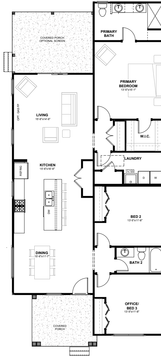
ONE STORY FLOOR PLAN
