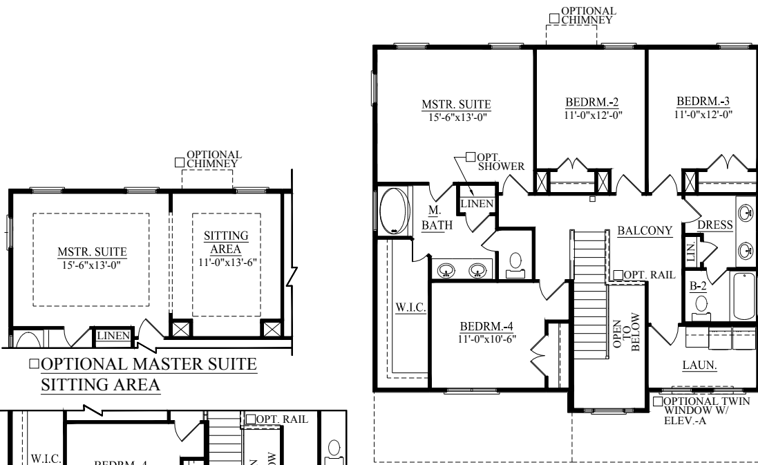
UPPER LEVEL PLAN FOR ELEVATIONS - A & B
