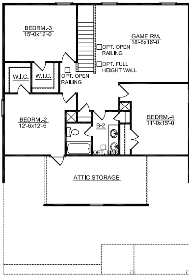
□ STANDARD FULL SECOND FLOOR PLAN W/ GAME RM.
