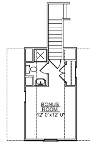
□ OPTIONAL BONUS RM. W/ OPTIONAL BATH @ A, B & C ELEV. (ADD 247 HTD. SQ. FT.)
