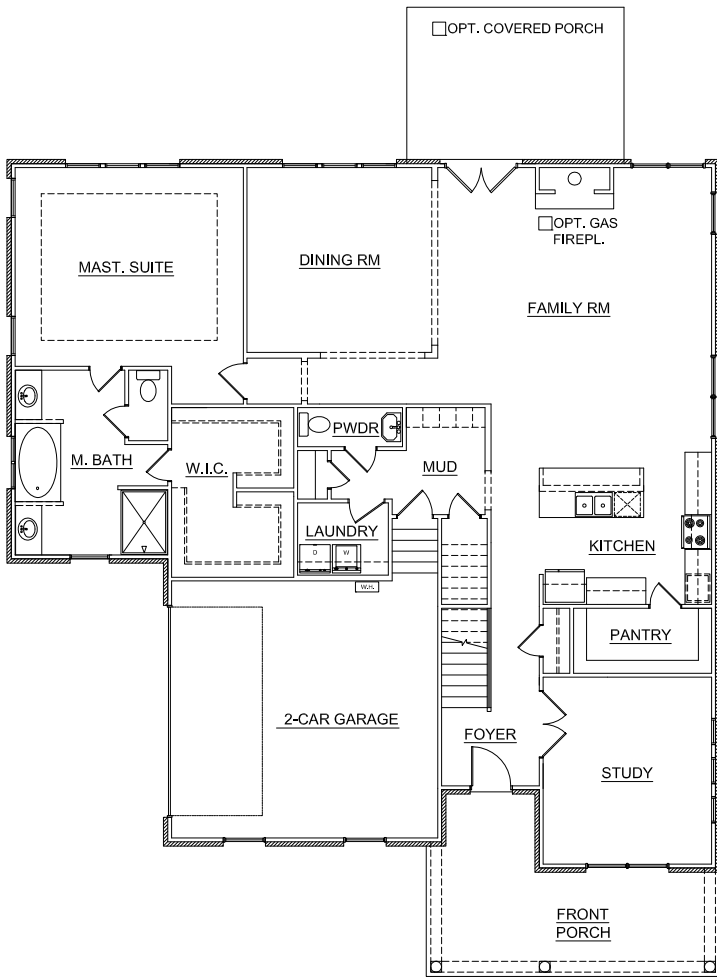
FIRST LEVEL PLAN
