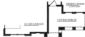
FLOOR PLAN- ELEVATION "C" w/ 3RD CAR GARAGE
