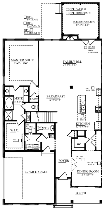
FIRST FLOOR PLAN ELEVATION "A"
