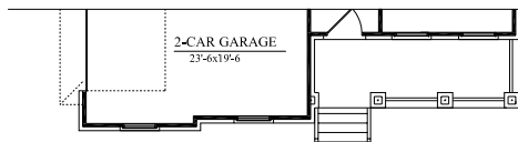
1ST FLOOR PLAN ELEVATION 'B'
