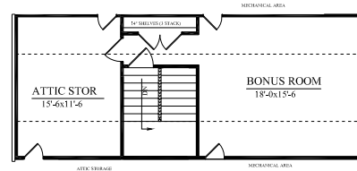
3RD FLOOR PLAN
