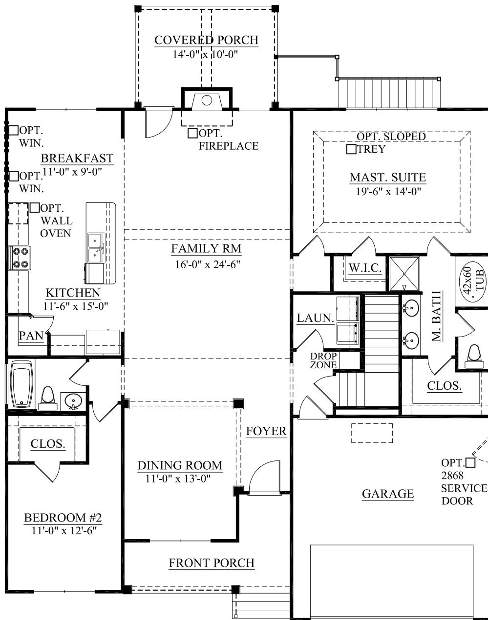
FIRST LEVEL PLAN
