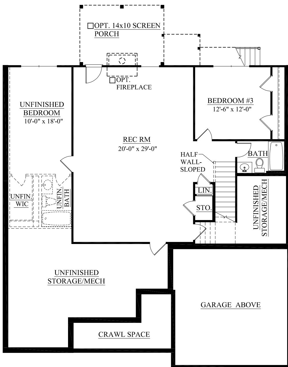
BASEMENT LEVEL PLAN
