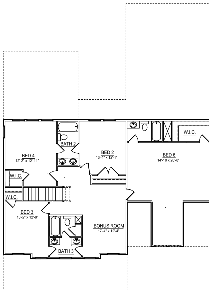
ELEVATION C - SECOND FLOOR PLAN
