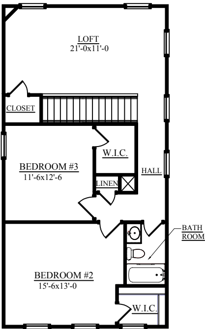
SECOND FLOOR PLAN STANDARD LAYOUT
