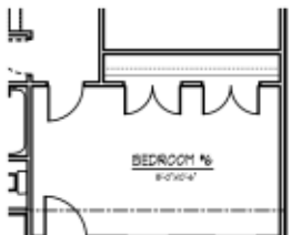
OPTIONAL SIXTH BEDROOM C
