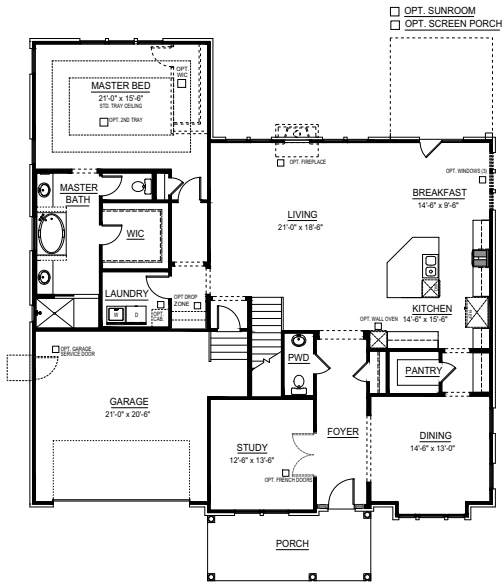
FIRST FLOOR PLAN - ELEVATION A
