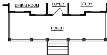
ELEVATION C-2 - FIRST FLOOR PLAN
