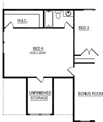
OPTIONAL BED 6 W/ BONUS ROOM
