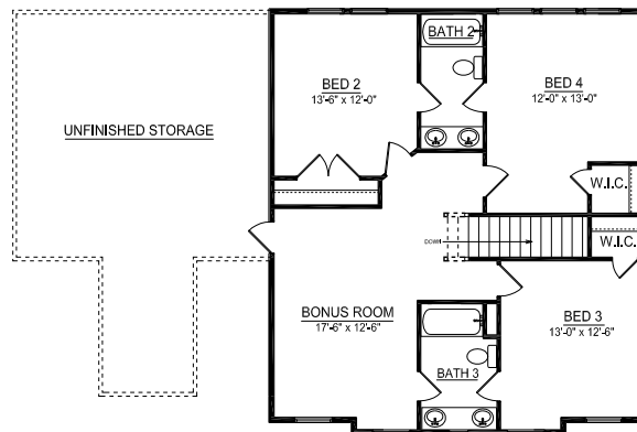
ELEVATION A/C - SECOND FLOOR PLAN
