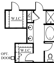
DELUXE M. BATH OPT. 2 W/ BONUS RM.
