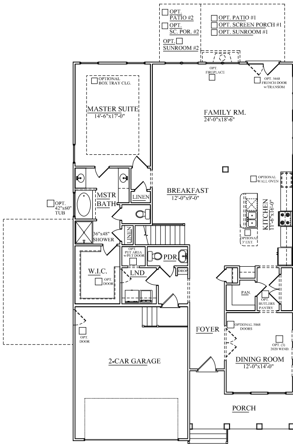
FIRST FLOOR PLAN ELEVATION "B"
