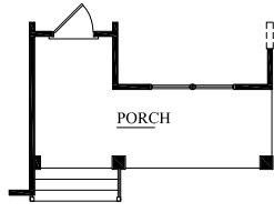
PORCH PLAN ELEVATION "D"
