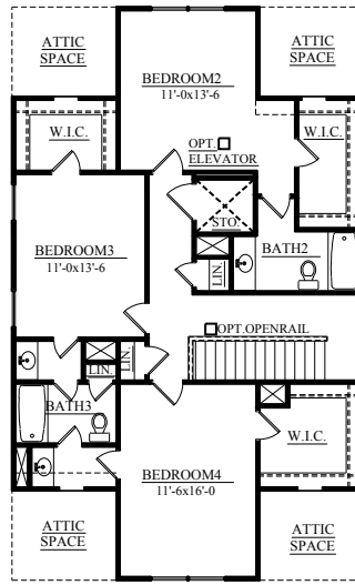
4TH BEDROOM UPPER LEVEL PLAN-OPT 2
