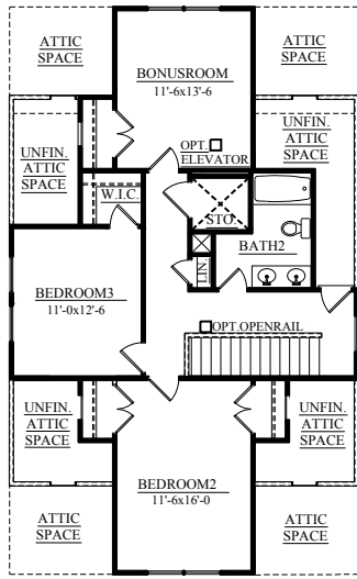
STANDARD UPPER LEVEL PLAN-ELEV. "A"
