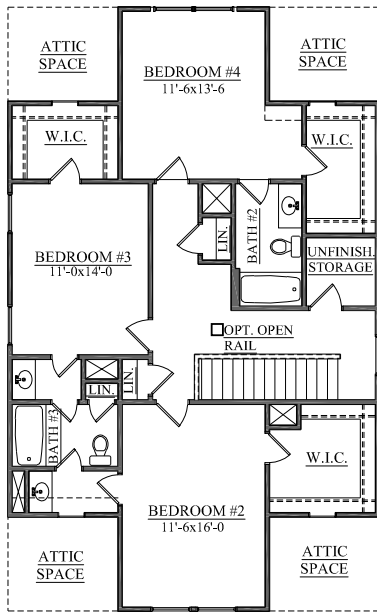
4TH BEDROOM UPPER LEVEL PLAN-OPT.#2
