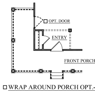
WRAP AROUND PORCH OPT.-A
