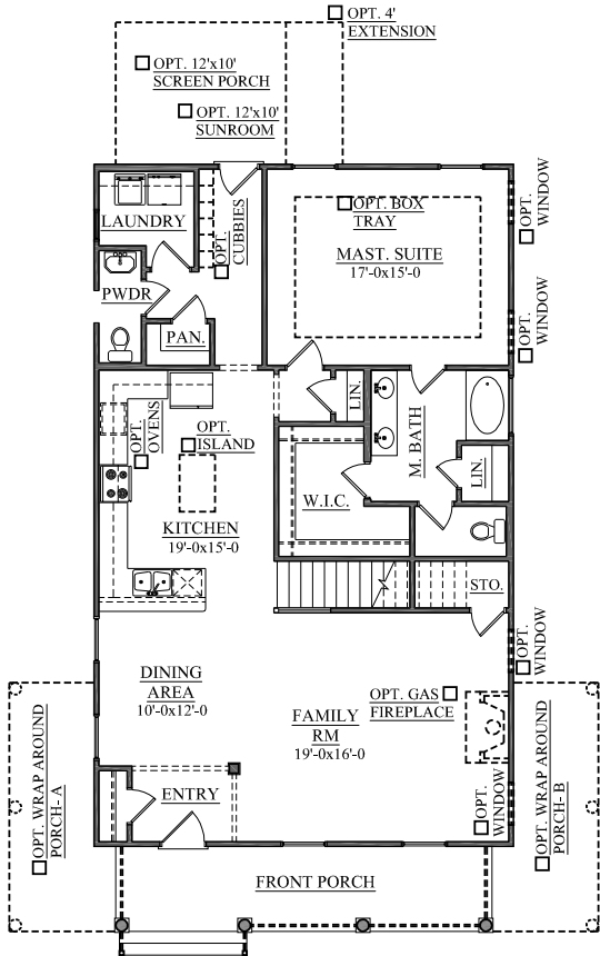
MAIN LEVEL PLAN-ELEV. "A","B"&"C"
