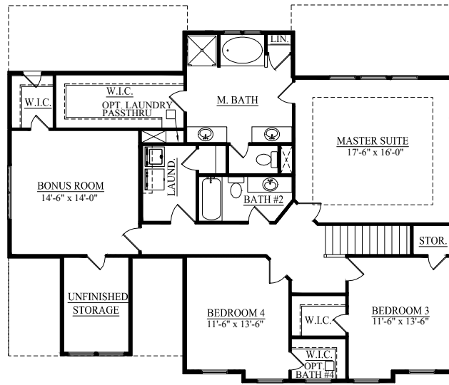
ELEVATION A - SECOND FLOOR PLAN
