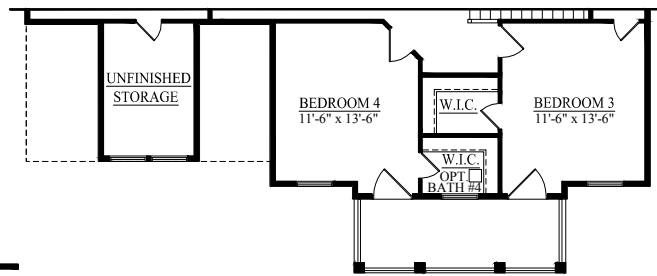
ELEVATION B - SECOND FLOOR PLAN
