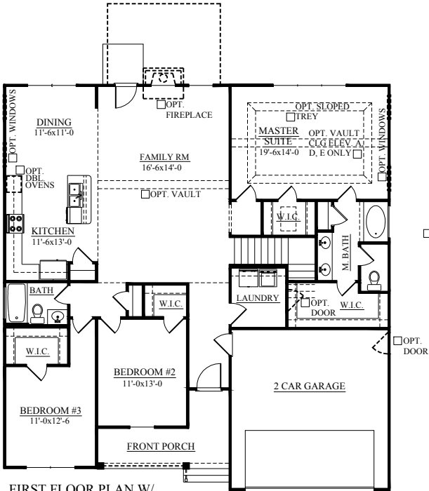
FIRST FLOOR PLAN W/ BONUS ROOM
