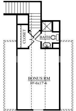
BONUS RM PLAN OPT. GUEST SUITE-ELEV. "D", "E", "F" ONLY
