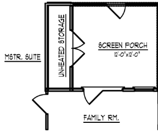
OPT. SCREEN PORCH SCALE 1/8" = 1'-0"
