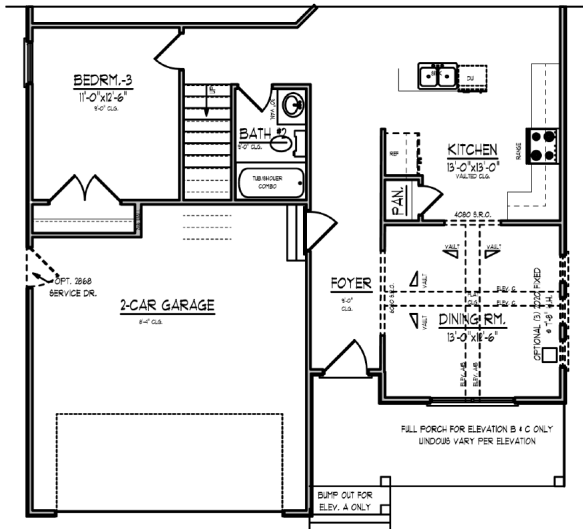
MAIN LEVEL PLAN ELEVATION (W/BONUS ROOM) SCALE 1/8" = 1'-0"
