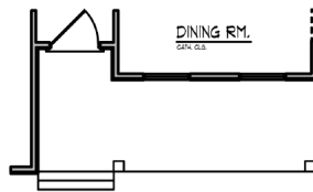
MAIN LEVEL PLAN ELEVATION C SCALE 1/8" = 1'-0"
