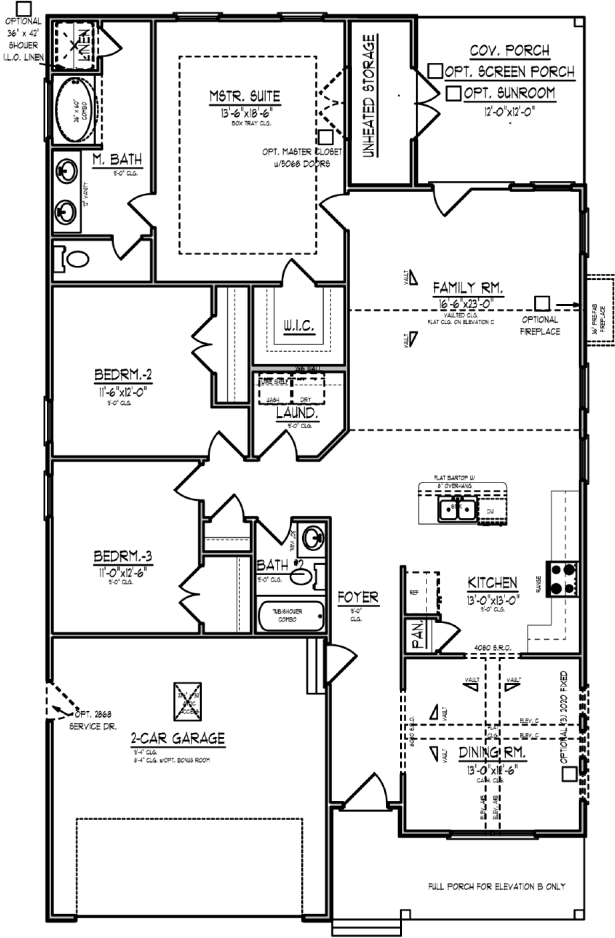
MAIN LEVEL PLAN ELEVATION A+B SCALE 1/8" = 1'-0"
