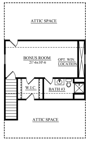
OPT. 3RD FLOOR GUEST SUITE
