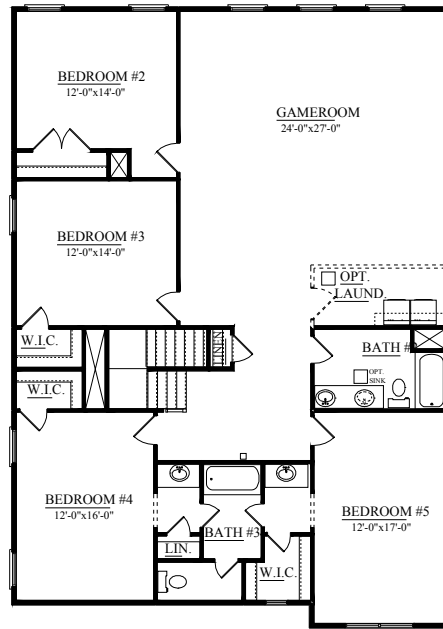
SECOND FLOOR PLAN ELEVATION A
