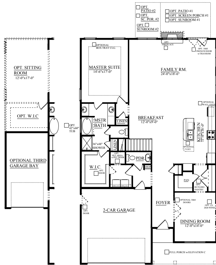
FIRST FLOOR PLAN ELEVATION "A&C"
