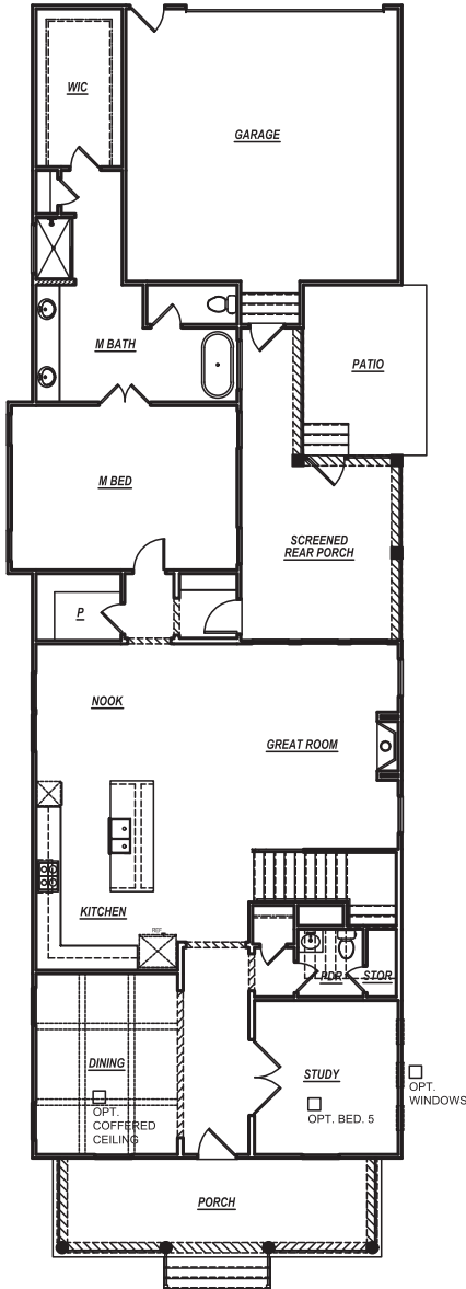
FIRST FLOOR PLAN ELEVATION A
