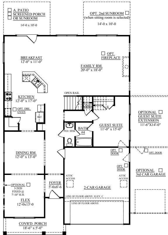
FIRST FLOOR PLAN ELEVATION "A" AND "B"
